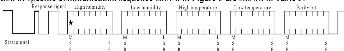
Figure 5: AM2305 single bus communication protocol
