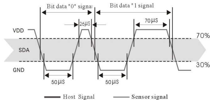
Figure 8: Single bus exploded timing diagram
